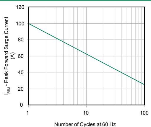
Figure 6 - Maximum Non-Repetitive Forward Surge Current
